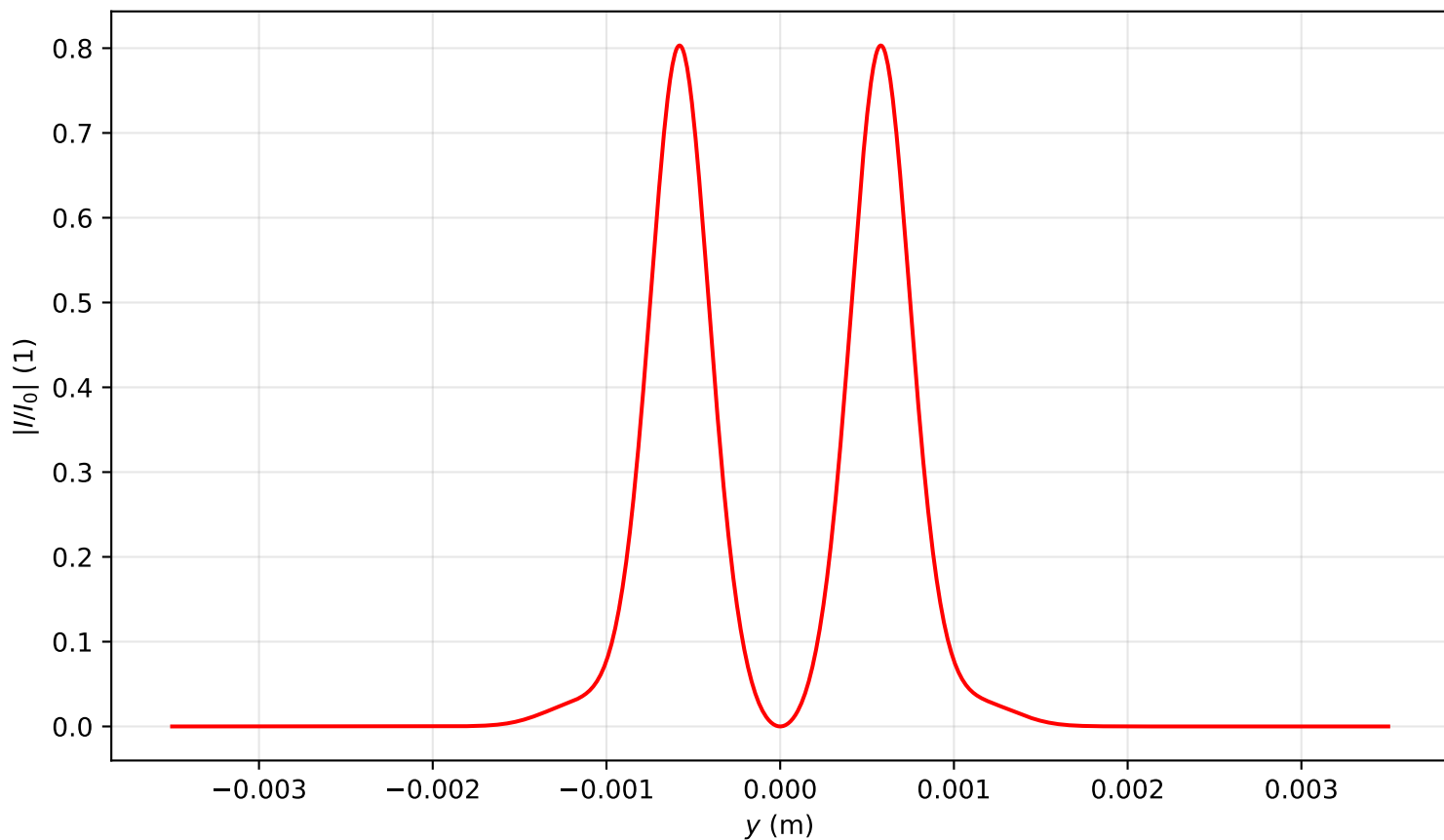
Intensity profile I(x=0, y, z=0.876)/I_0 , P_{in}=4.0P_{cr} , artificial time
